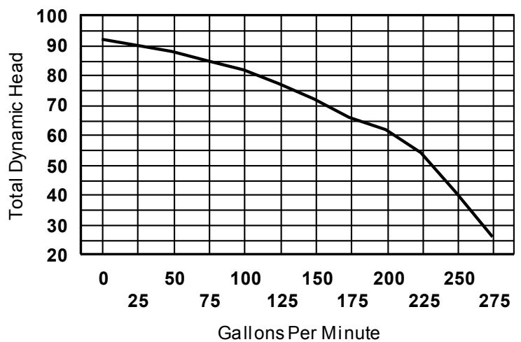
Piranha pump model PSS-750 7.5 hp, 230v/460v, 3 phase
