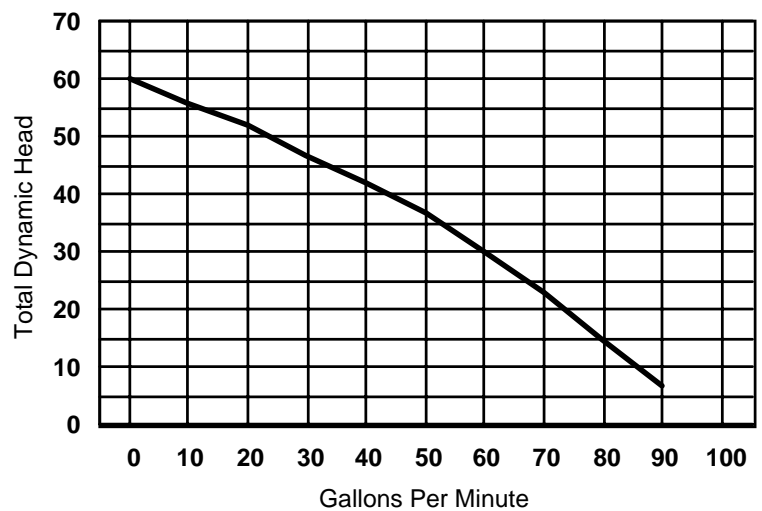
Piranha Model P-100-SS 1 hp 115v 1ph
