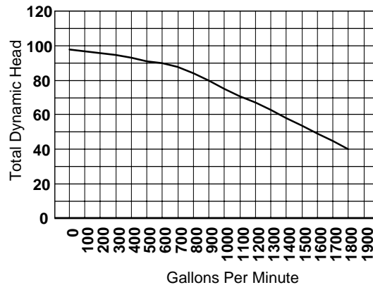
Piranha Agitator Pump Severe Duty Model P-50-A
